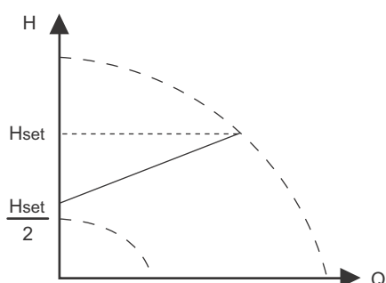
Fig. 52 "Proportional pressure"
