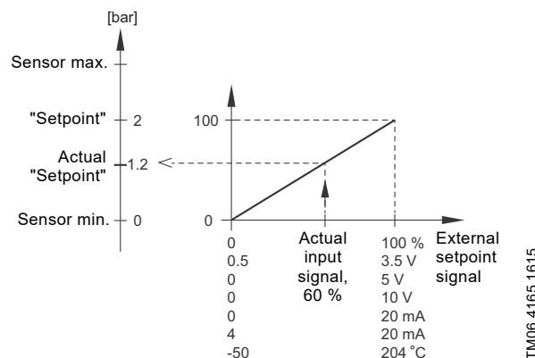
Fig. 75 Example of setpoint influence with sensor feedback
