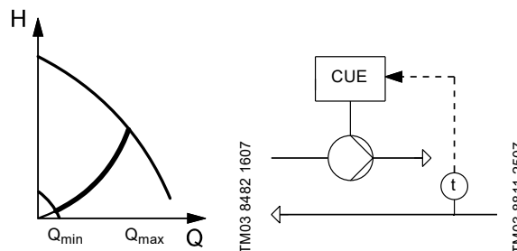
Fig. 104 Constant temperature
