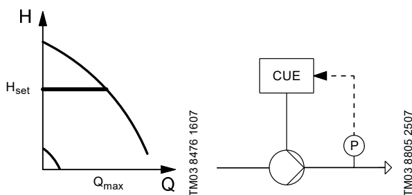
Fig. 89 Constant pressure
