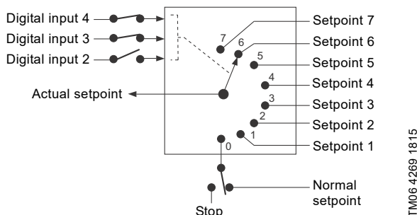
Fig. 80 Principle sketch showing how predefined setpoints function
