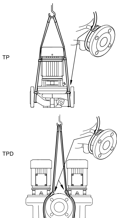
Fig. 1 Lifting the pump by means of nylon straps
