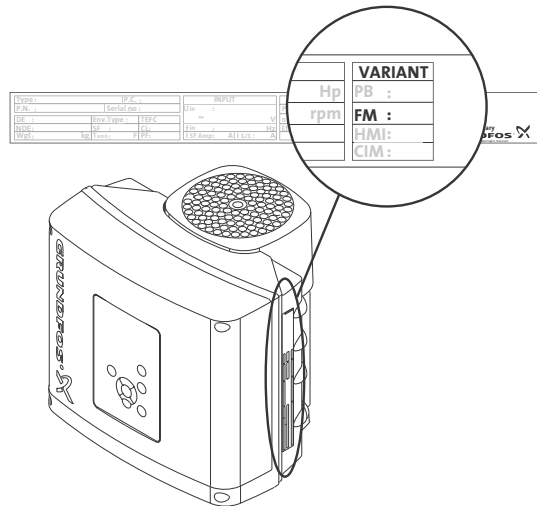
Fig. 151 Identification of functional module
