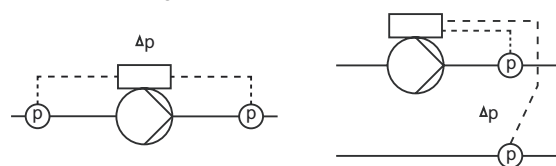
Fig. 59 "Constant differential pressure"
