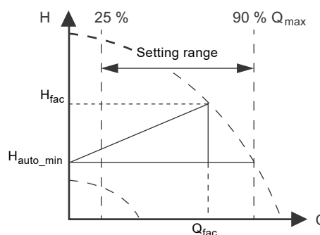
Fig. 51 FLOW ADAPT
