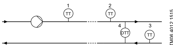
Fig. 70 Overview of Pt100/1000 sensor locations
