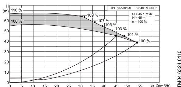
Fig. 17 TPE and TPED pumps with extended performance range
