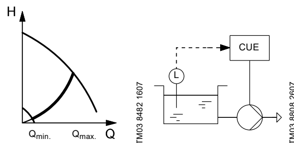
Fig. 101 Constant level
