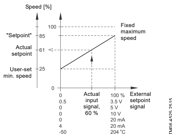
Fig. 76 Example of setpoint influence with constant curve
