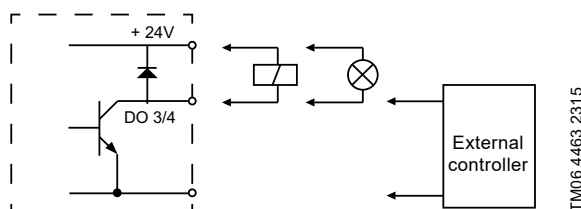
Fig. 72 Example of configurable digital inputs or outputs
