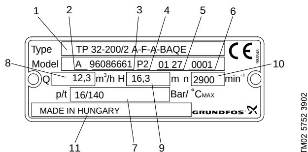
Fig. 1 Example of nameplate
