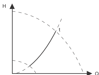
Fig. 56 "Constant temperature"
