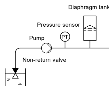
Fig. 92 Position of the non-return valve and pressure sensor in a system with suction lift
