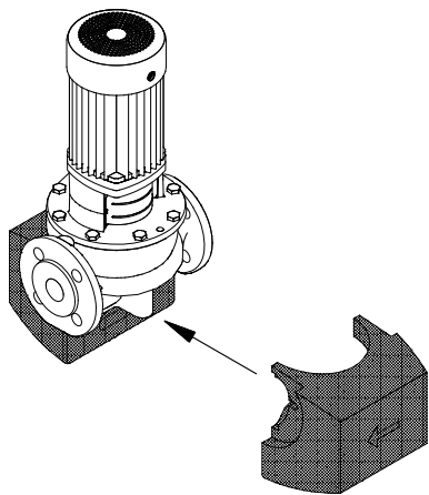
Fig. 175 Insulating kit
