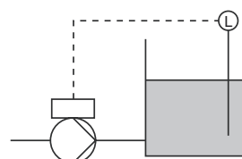
Fig. 65 Constant level
