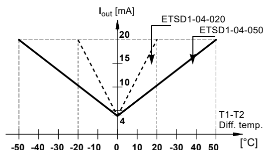
Fig. 177 Sensor characteristics
