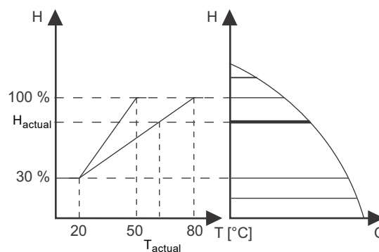
Fig. 81 "Temperature influence"
